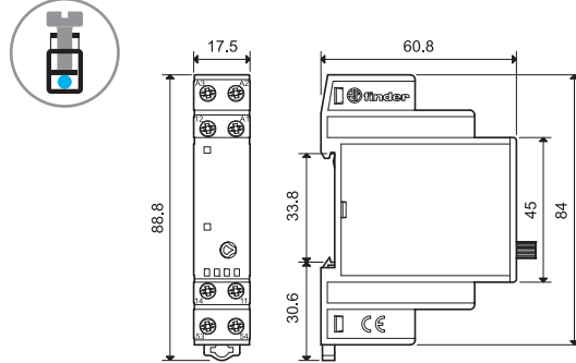
Type 19.41 Screw terminal
