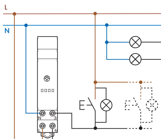
4 wire connection
