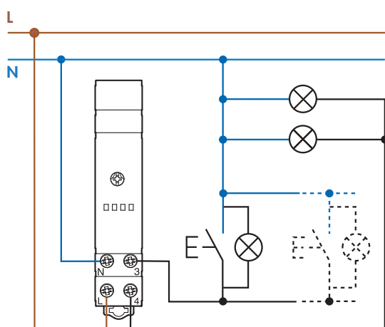
3 wire connection
